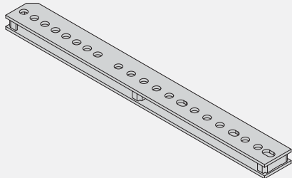
Adjustable waling extension FF20/50
